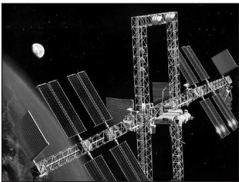
Space Station Freedom (Source: 90-Day Study)
