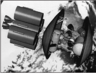
Mars Transfer Vehicle would have propelled crew and Mars excursion vehicle to Mars orbit (Source: 90-Day Study)
