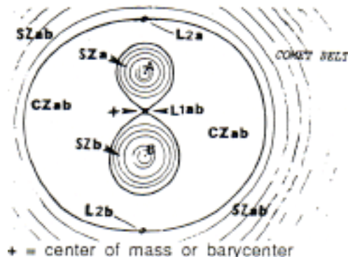
Fig.3 Stable vs. Chaotic Orbits around Binaries
