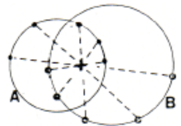
Fig. 1. + = center of mass or barycenter of system.
