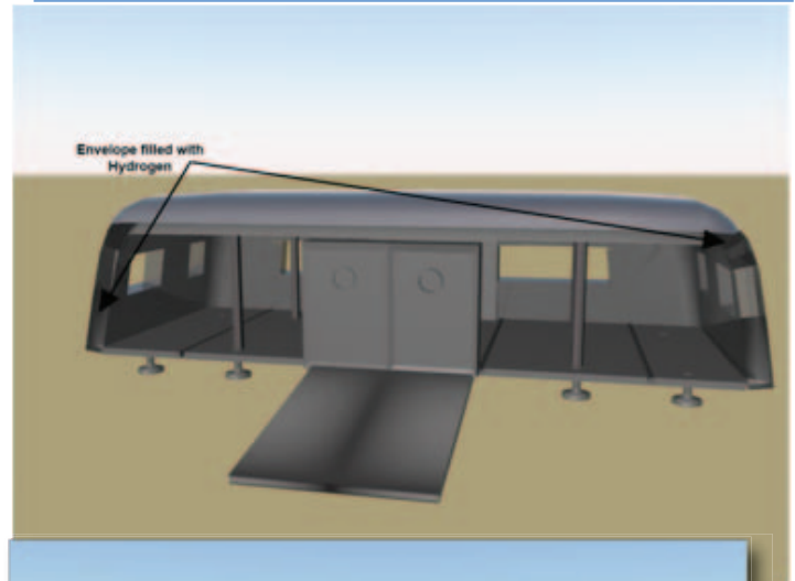
Figure 2.5.1 fully constructed Rapid Assembly Mars Settlement, providing a solid work and research base for four people for up to sixty days
