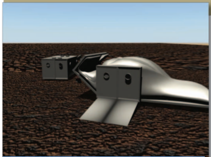
Figure 2.5.2 RAMS in the first stages of construction, once the floor has been secured the base will proceed to inflate and become fully inhabitable.
